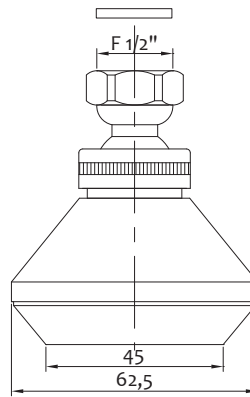
Soffione doccia in ottone cromato con ugelli in gomma Chrome plated brass shower head with rubber nozzles
