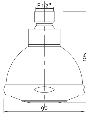
Soffione ABS cromata 5 getti Chrome ABS shower head 5 water jet
