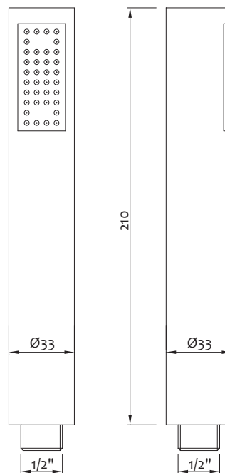
Doccetta in BAS cromata "PHONE" ABS chromed hand shower "PHONE"
